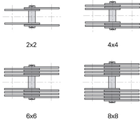
Plate lacing Laschenkombination
